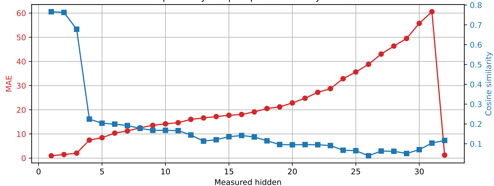
SmolLM2-360M | Prompt 3 Spared layer 4 | Unquantized vs hybrid
