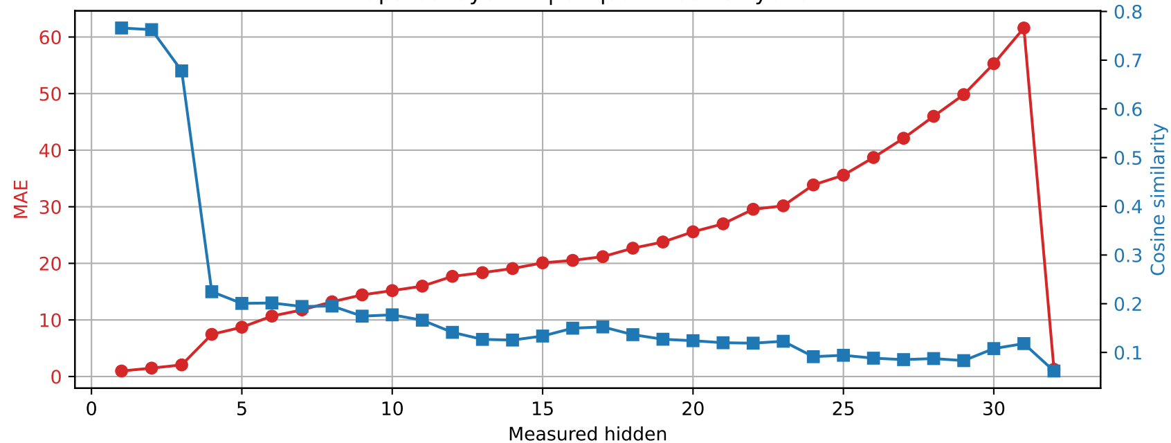
SmolLM2-360M | Prompt 3 Spared layer 22 | Unquantized vs hybrid
