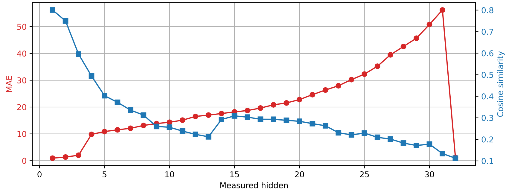
SmolLM2-360M | Prompt 4 Spared layer 5 | Unquantized vs hybrid
