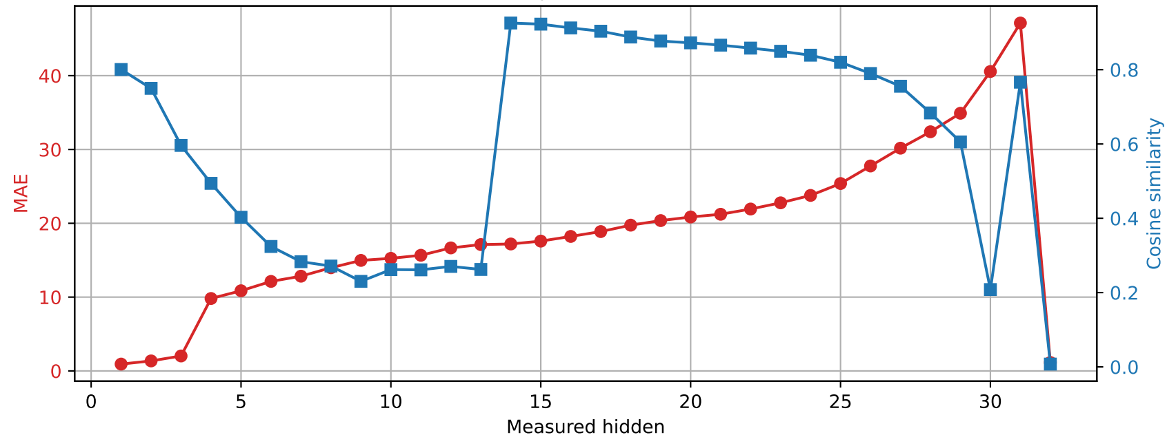
SmolLM2-360M | Prompt 4 Spared layer 9 | Unquantized vs hybrid
