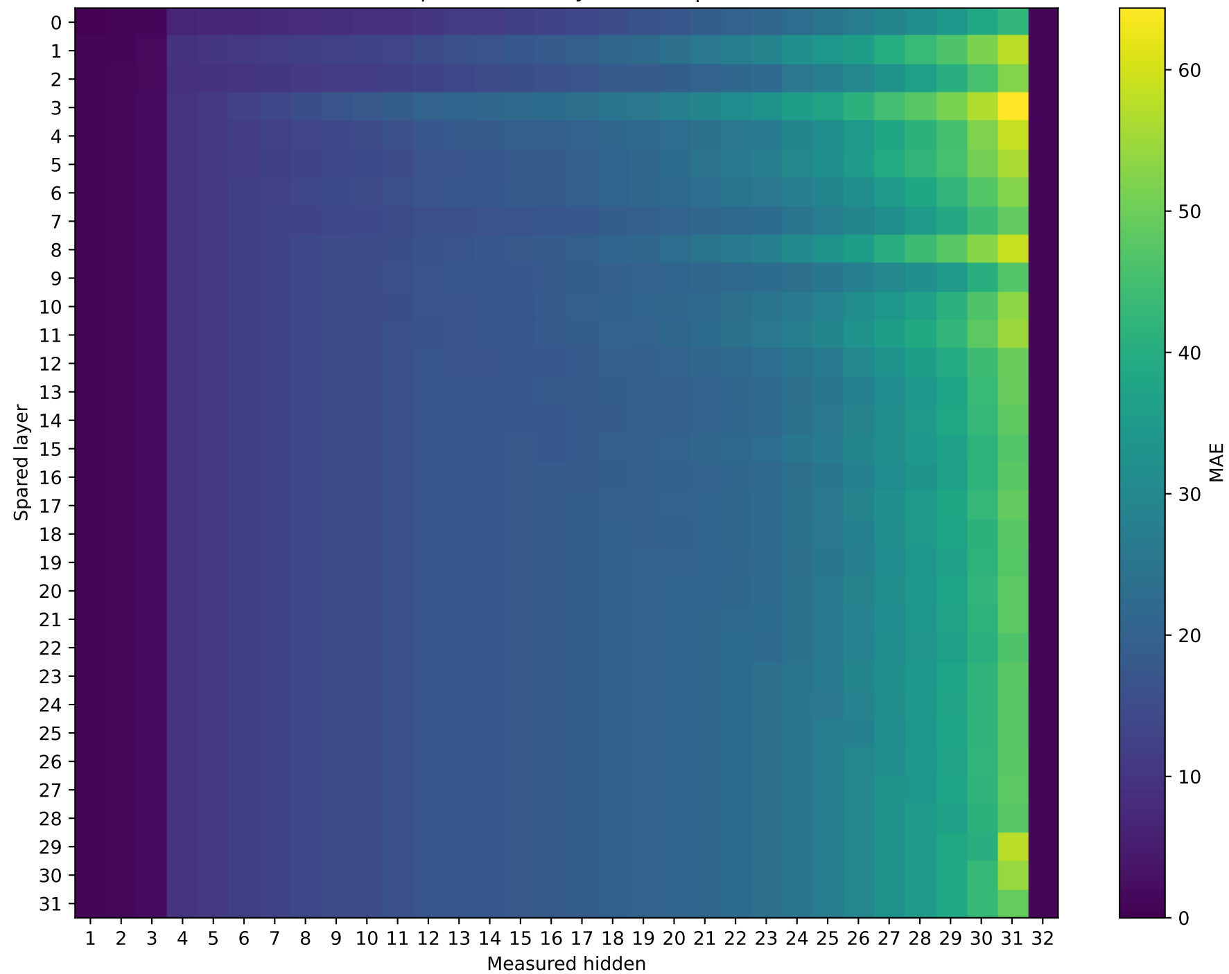
SmolLM2-360M | Prompt 4 Unquantized vs hybrid MAE | int4
