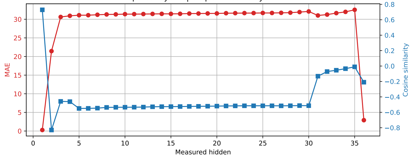
Qwen2.5-3B | Prompt 0 Spared layer 7 | Unquantized vs hybrid
