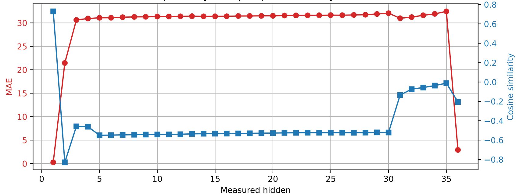
Qwen2.5-3B | Prompt 0 Spared layer 13 | Unquantized vs hybrid
