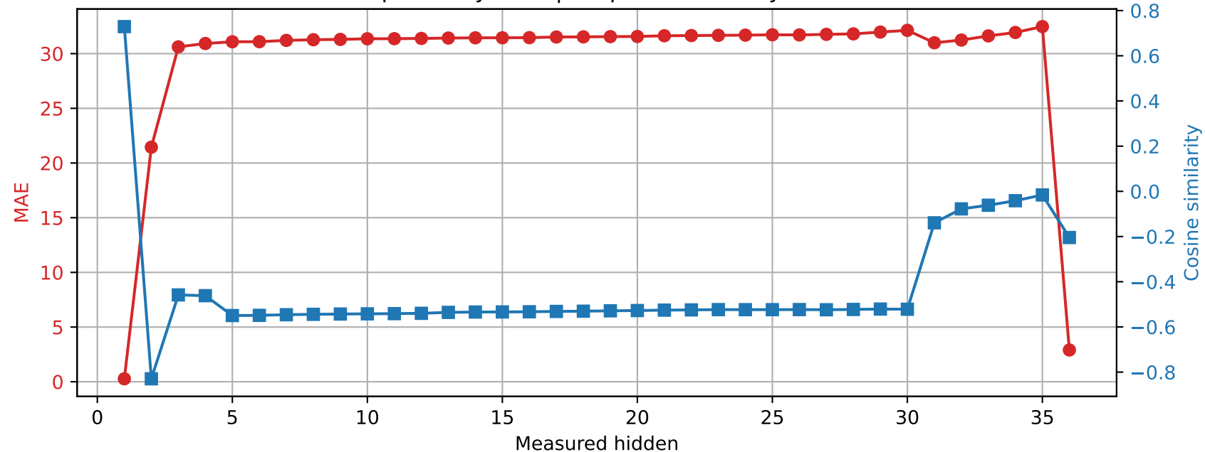
Qwen2.5-3B | Prompt 0 Spared layer 30 | Unquantized vs hybrid
