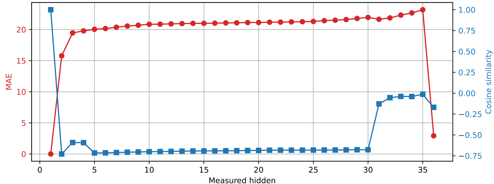
Qwen2.5-3B | Prompt 1 Spared layer 0 | Unquantized vs hybrid
