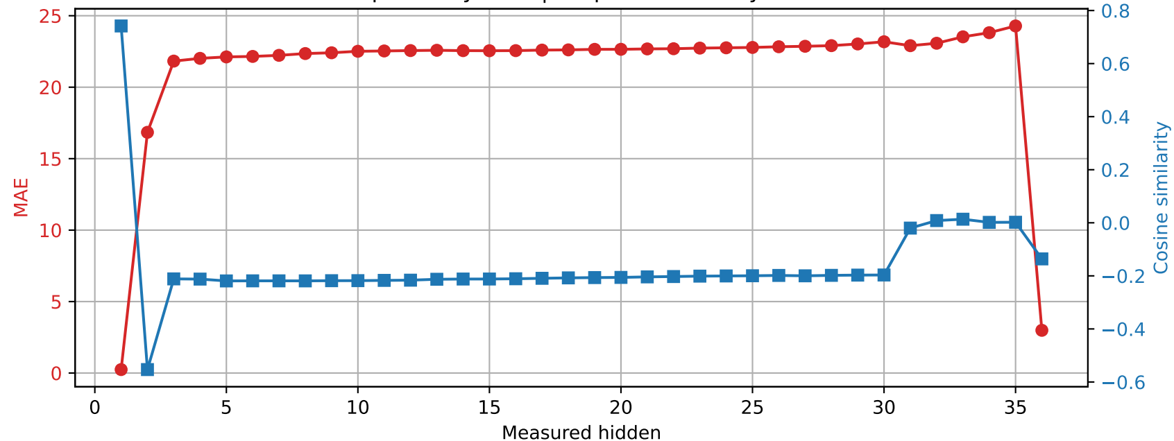
Qwen2.5-3B | Prompt 1 Spared layer 13 | Unquantized vs hybrid
