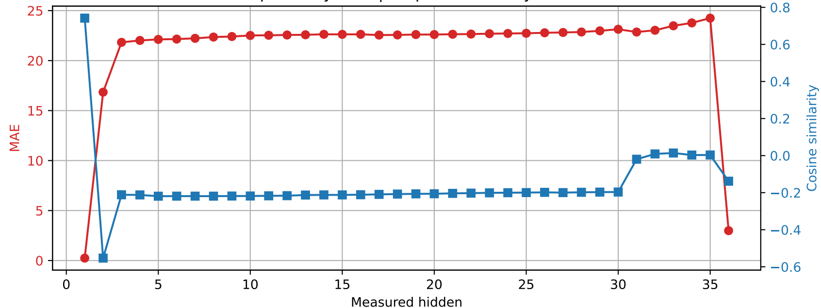
Qwen2.5-3B | Prompt 1 Spared layer 16 | Unquantized vs hybrid
