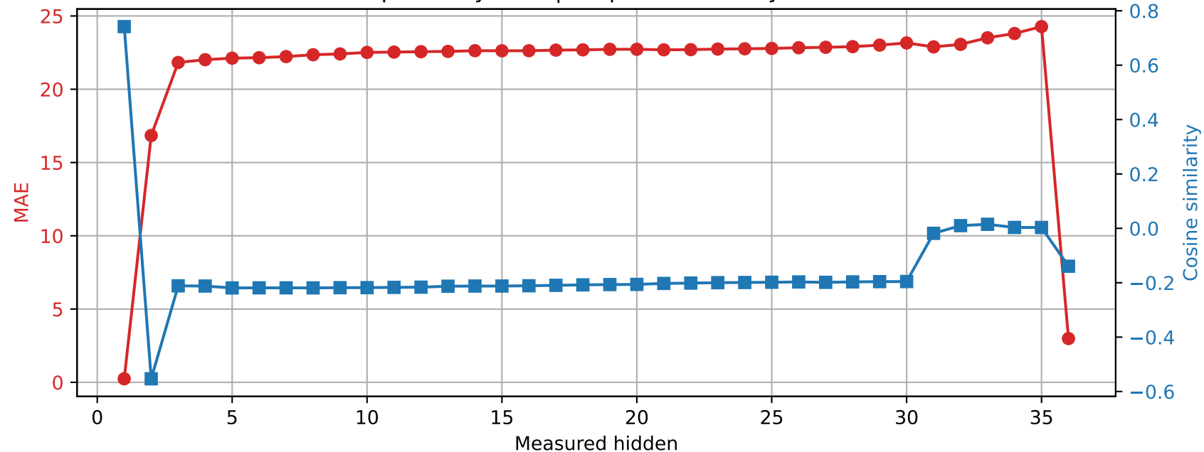
Qwen2.5-3B | Prompt 1 Spared layer 20 | Unquantized vs hybrid
