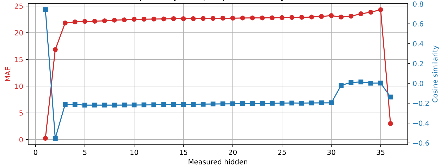
Qwen2.5-3B | Prompt 1 Spared layer 22 | Unquantized vs hybrid
