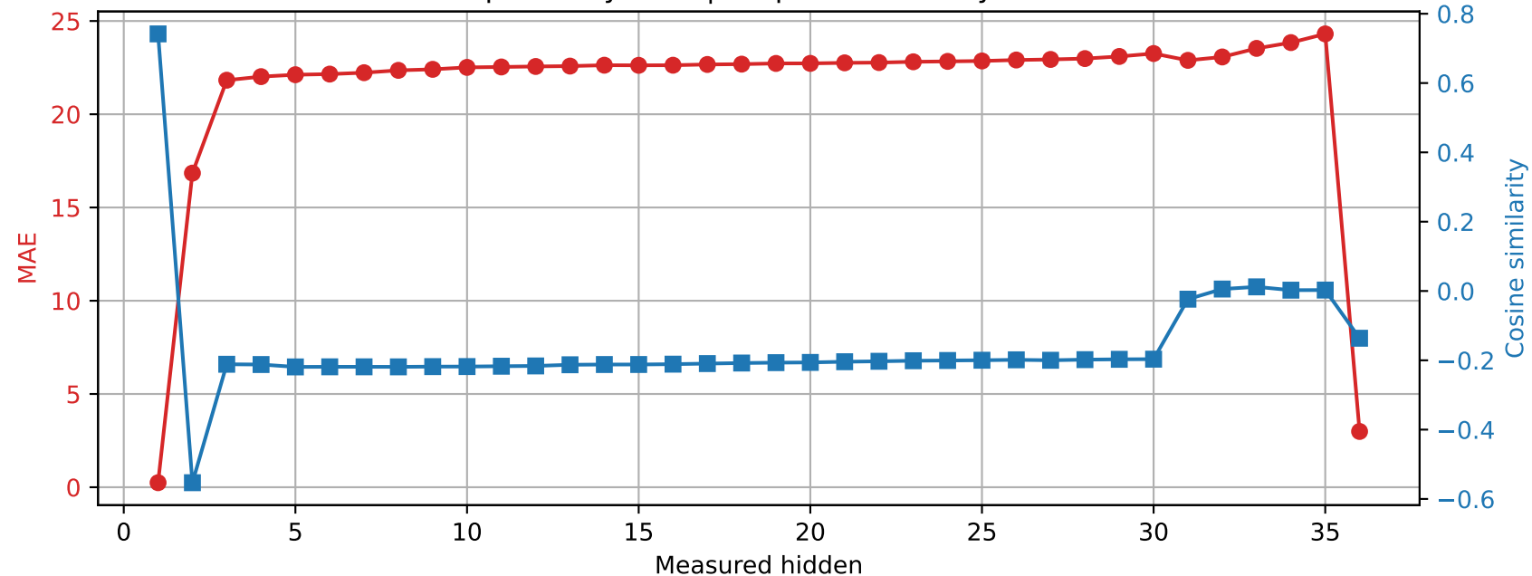
Qwen2.5-3B | Prompt 1 Spared layer 30 | Unquantized vs hybrid
