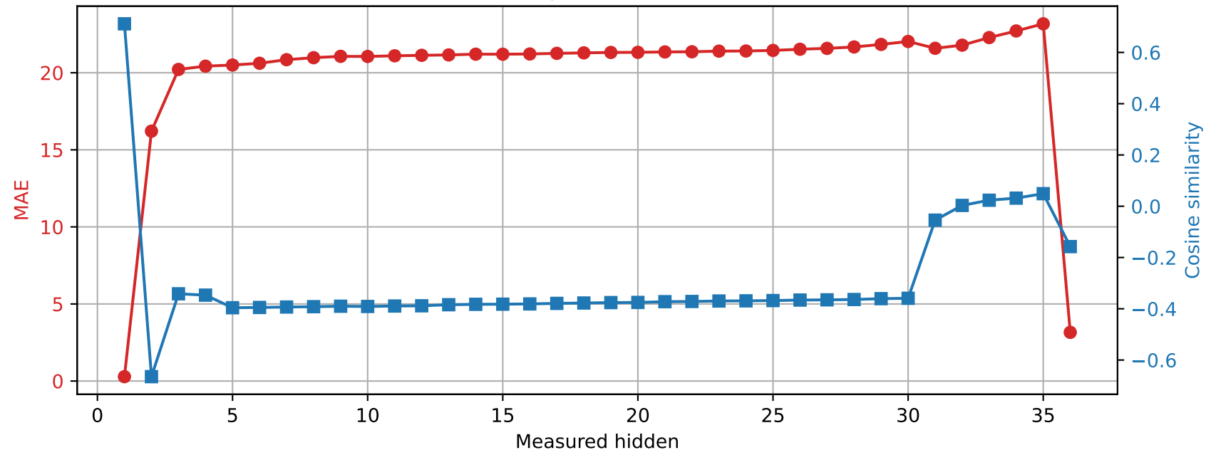
Qwen2.5-3B | Prompt 2 Spared layer 9 | Unquantized vs hybrid
