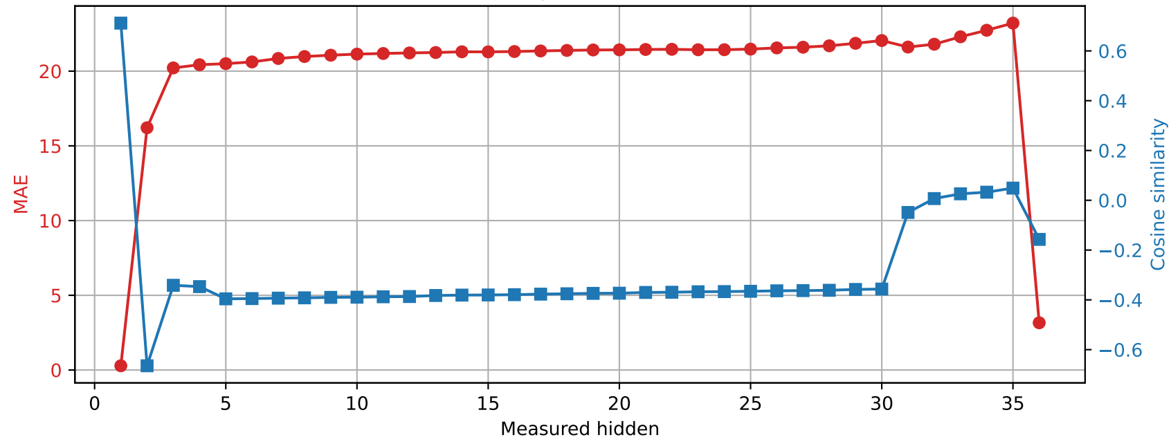
Qwen2.5-3B | Prompt 2 Spared layer 22 | Unquantized vs hybrid
