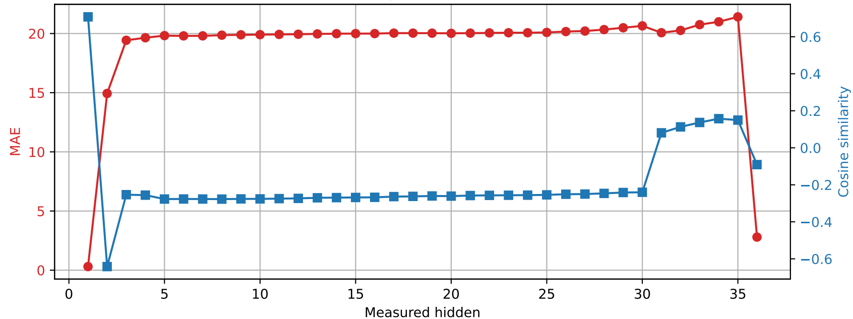
Qwen2.5-3B | Prompt 3 Spared layer 4 | Unquantized vs hybrid
