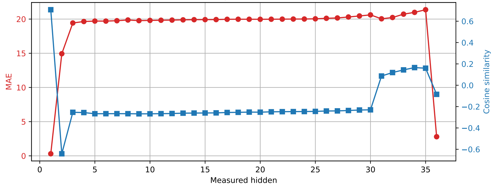
Qwen2.5-3B | Prompt 3 Spared layer 8 | Unquantized vs hybrid
