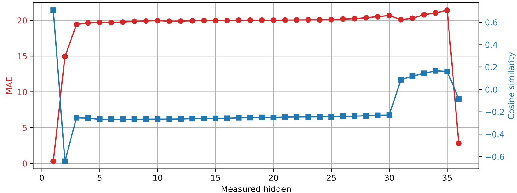
Qwen2.5-3B | Prompt 3 Spared layer 10 | Unquantized vs hybrid
