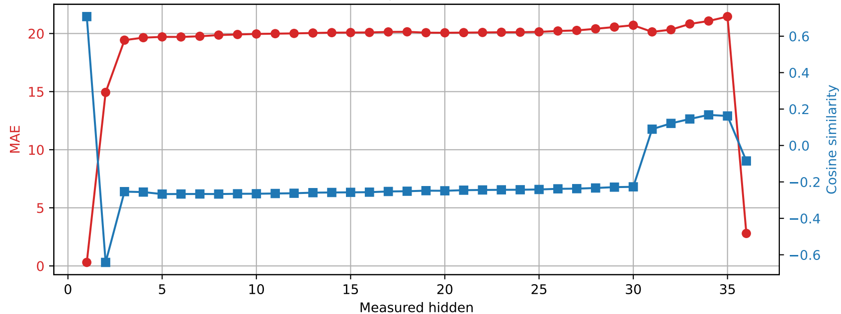
Qwen2.5-3B | Prompt 3 Spared layer 18 | Unquantized vs hybrid
