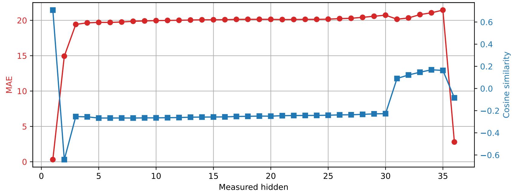
Qwen2.5-3B | Prompt 3 Spared layer 20 | Unquantized vs hybrid
