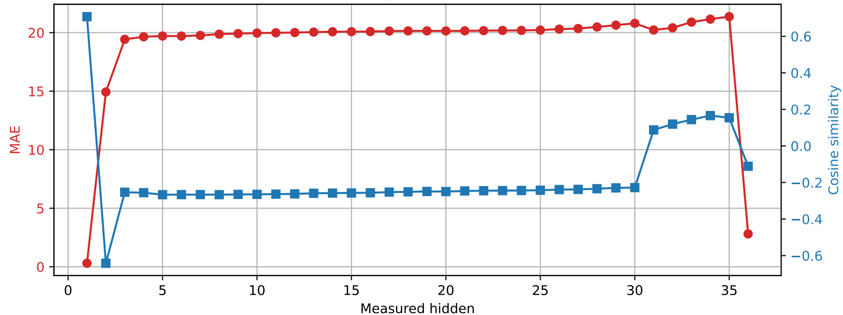
Qwen2.5-3B | Prompt 3 Spared layer 34 | Unquantized vs hybrid
