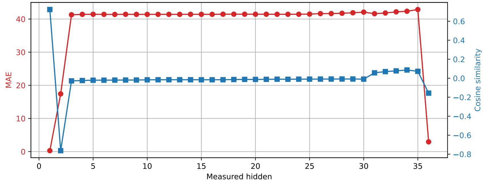
Qwen2.5-3B | Prompt 4 Spared layer 2 | Unquantized vs hybrid
