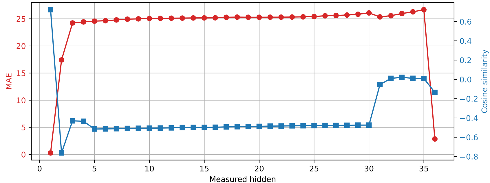
Qwen2.5-3B | Prompt 4 Spared layer 18 | Unquantized vs hybrid
