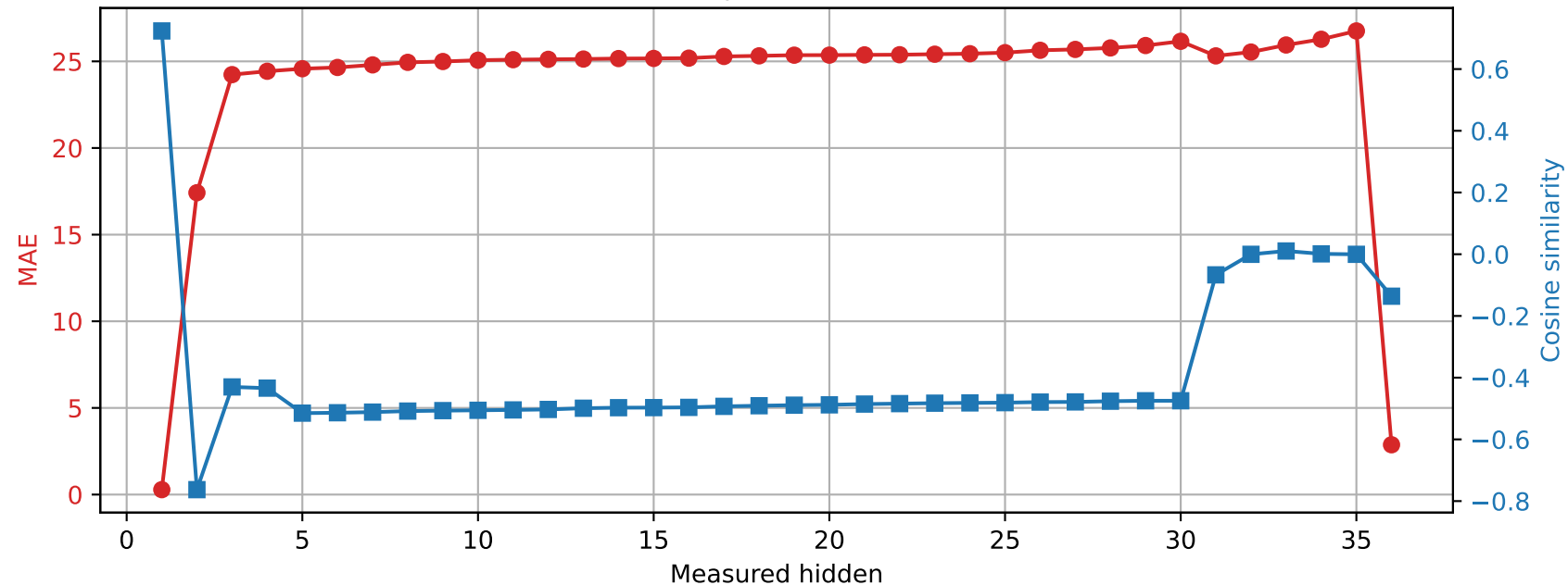
Qwen2.5-3B | Prompt 4 Spared layer 30 | Unquantized vs hybrid
