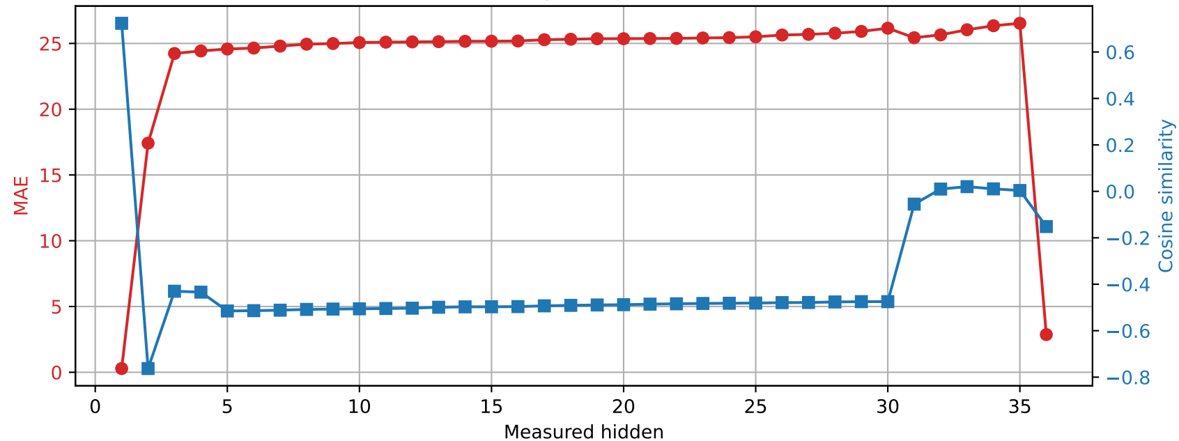
Qwen2.5-3B | Prompt 4 Spared layer 34 | Unquantized vs hybrid
