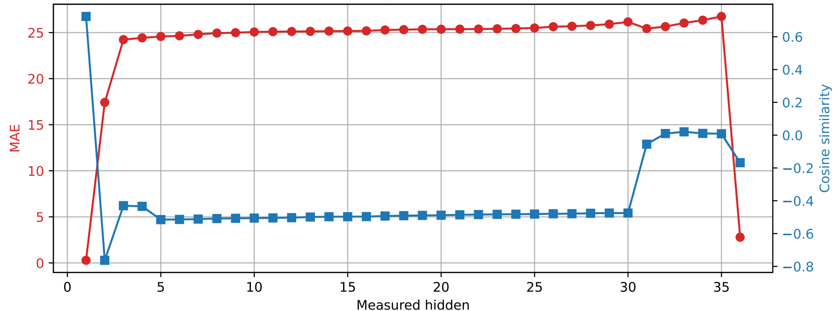
Qwen2.5-3B | Prompt 4 Spared layer 35 | Unquantized vs hybrid
