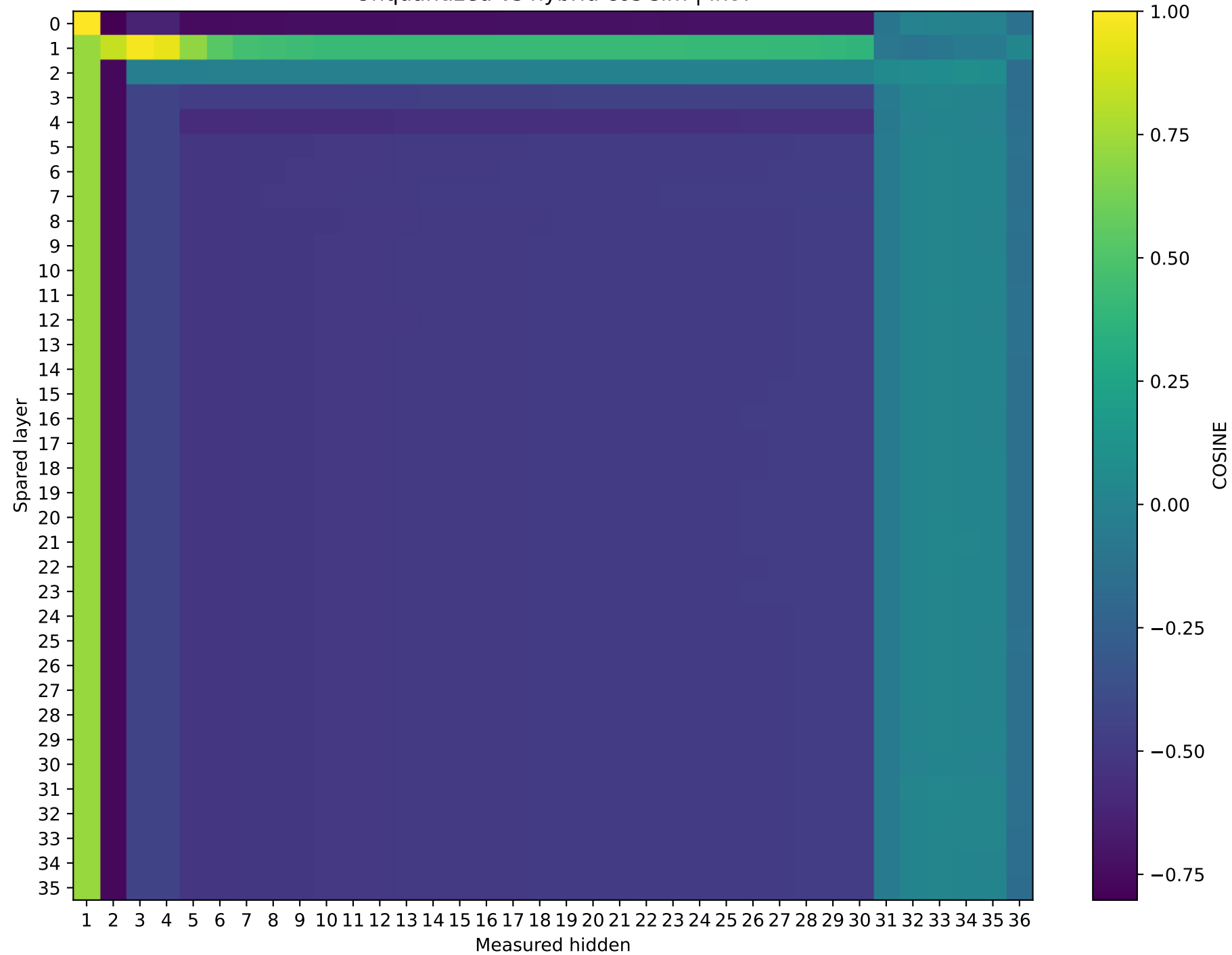
Qwen2.5-3B | Prompt 4 Unquantized vs hybrid cos sim | int4
