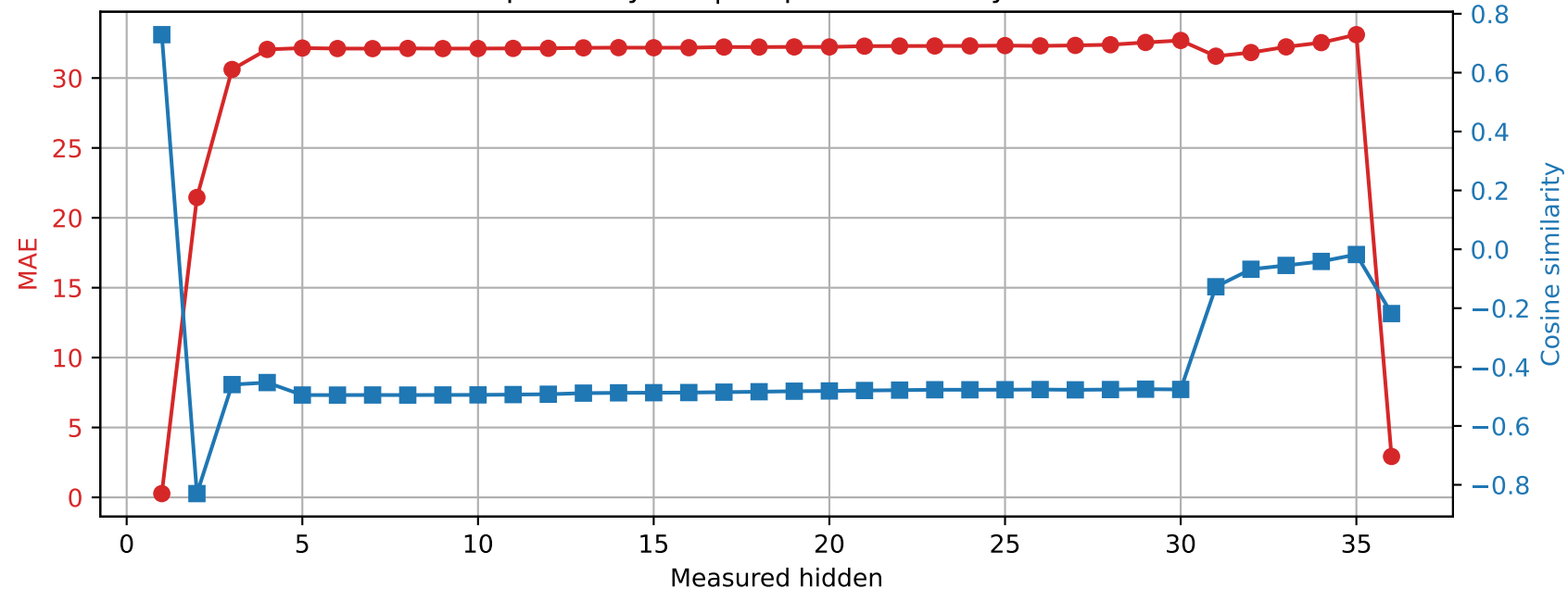
Qwen2.5-3B | Prompt 0 Spared layer 3 | Unquantized vs hybrid
