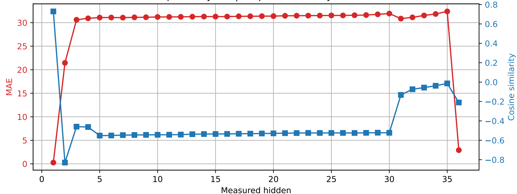
Qwen2.5-3B | Prompt 0 Spared layer 6 | Unquantized vs hybrid
