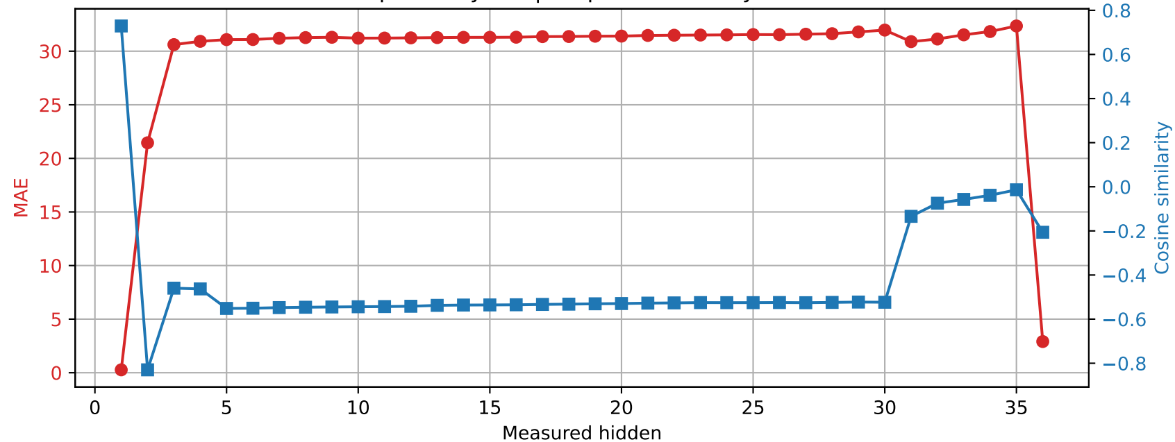
Qwen2.5-3B | Prompt 0 Spared layer 9 | Unquantized vs hybrid
