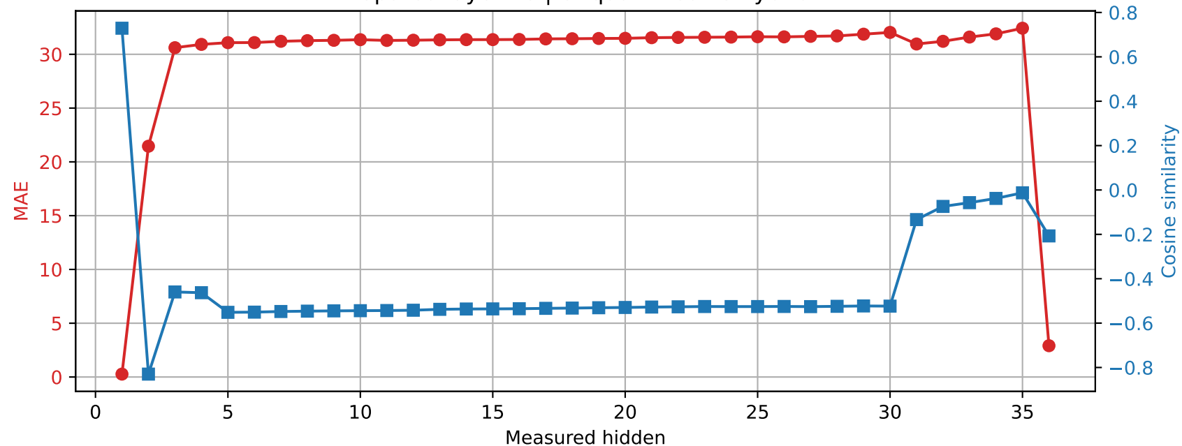
Qwen2.5-3B | Prompt 0 Spared layer 10 | Unquantized vs hybrid
