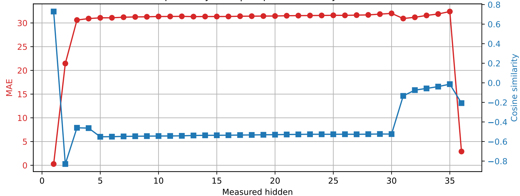
Qwen2.5-3B | Prompt 0 Spared layer 12 | Unquantized vs hybrid
