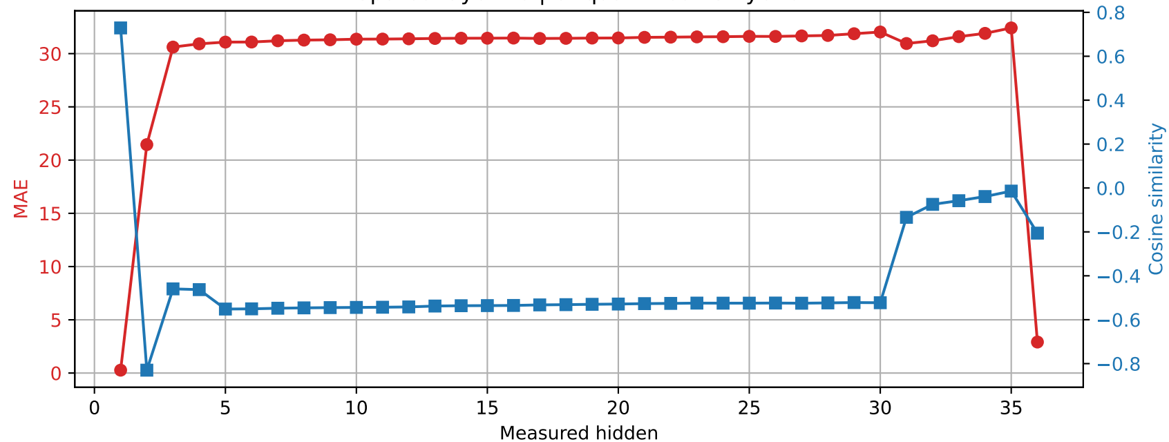
Qwen2.5-3B | Prompt 0 Spared layer 16 | Unquantized vs hybrid
