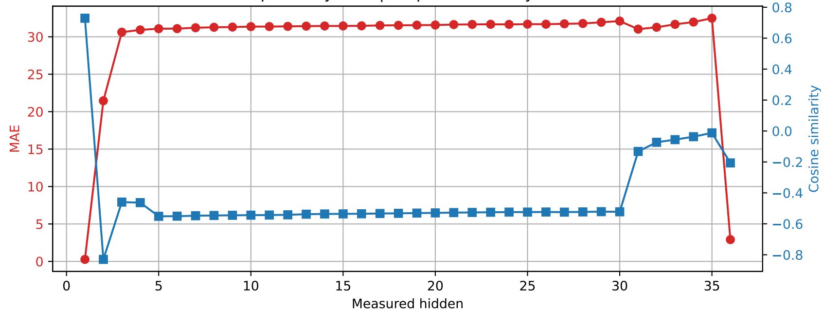
Qwen2.5-3B | Prompt 0 Spared layer 23 | Unquantized vs hybrid
