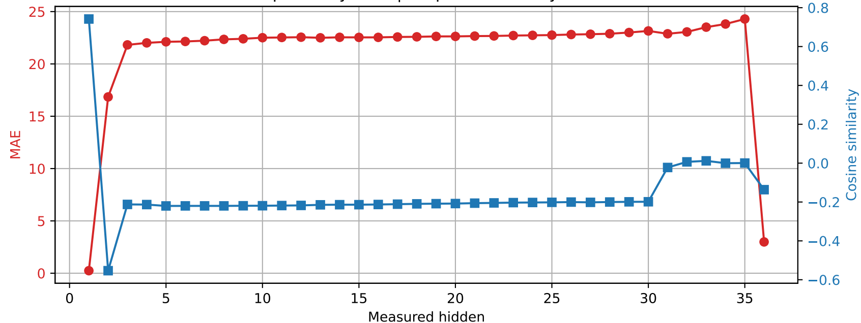
Qwen2.5-3B | Prompt 1 Spared layer 12 | Unquantized vs hybrid
