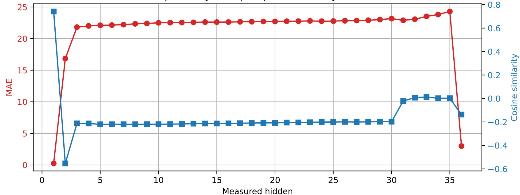
Qwen2.5-3B | Prompt 1 Spared layer 23 | Unquantized vs hybrid
