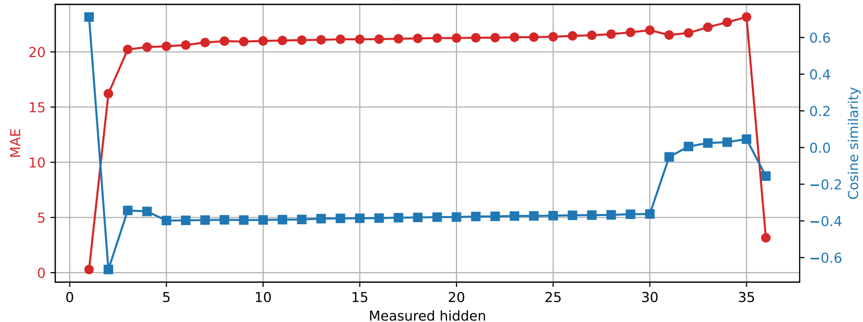
Qwen2.5-3B | Prompt 2 Spared layer 8 | Unquantized vs hybrid
