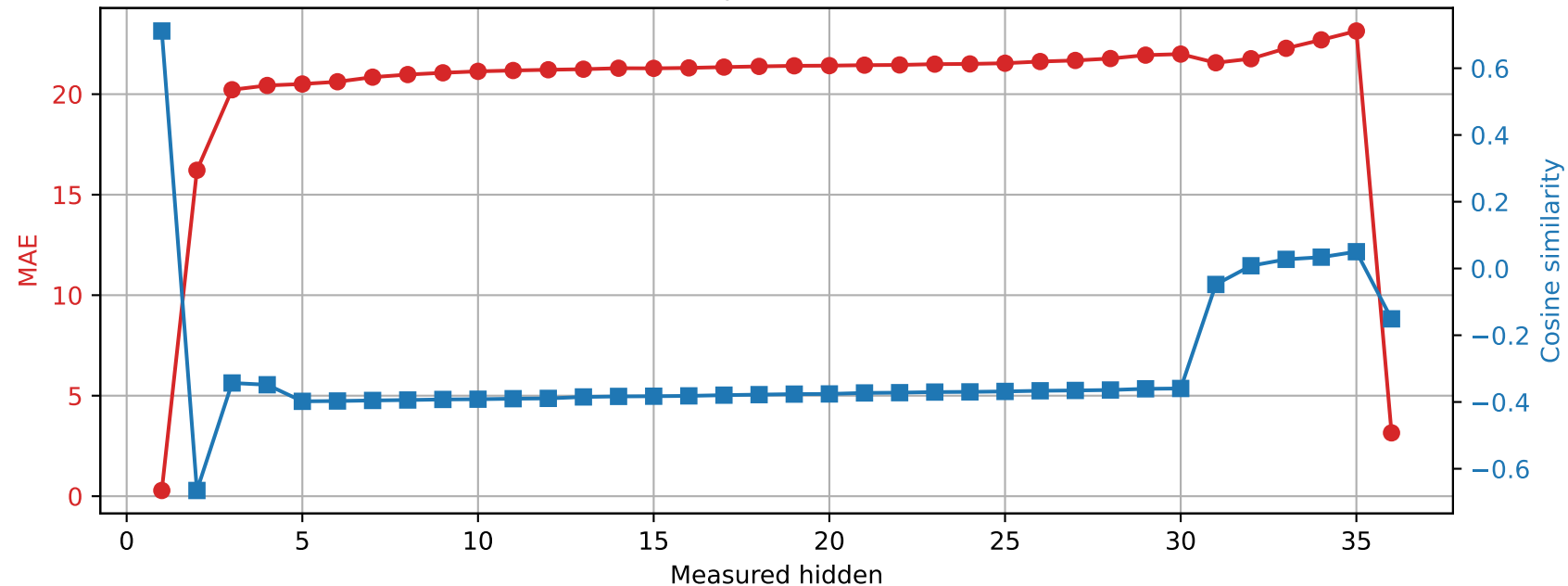
Qwen2.5-3B | Prompt 2 Spared layer 29 | Unquantized vs hybrid
