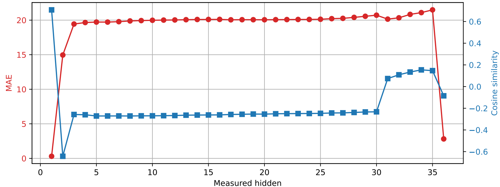
Qwen2.5-3B | Prompt 3 Spared layer 16 | Unquantized vs hybrid
