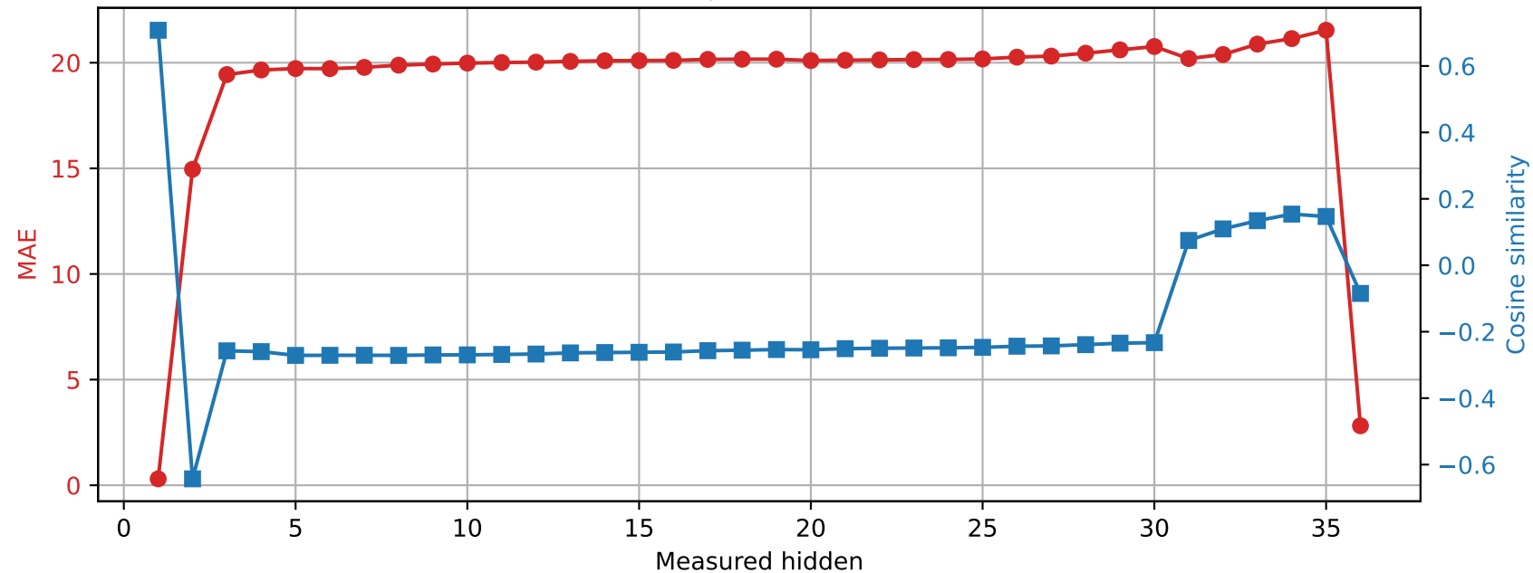
Qwen2.5-3B | Prompt 3 Spared layer 19 | Unquantized vs hybrid
