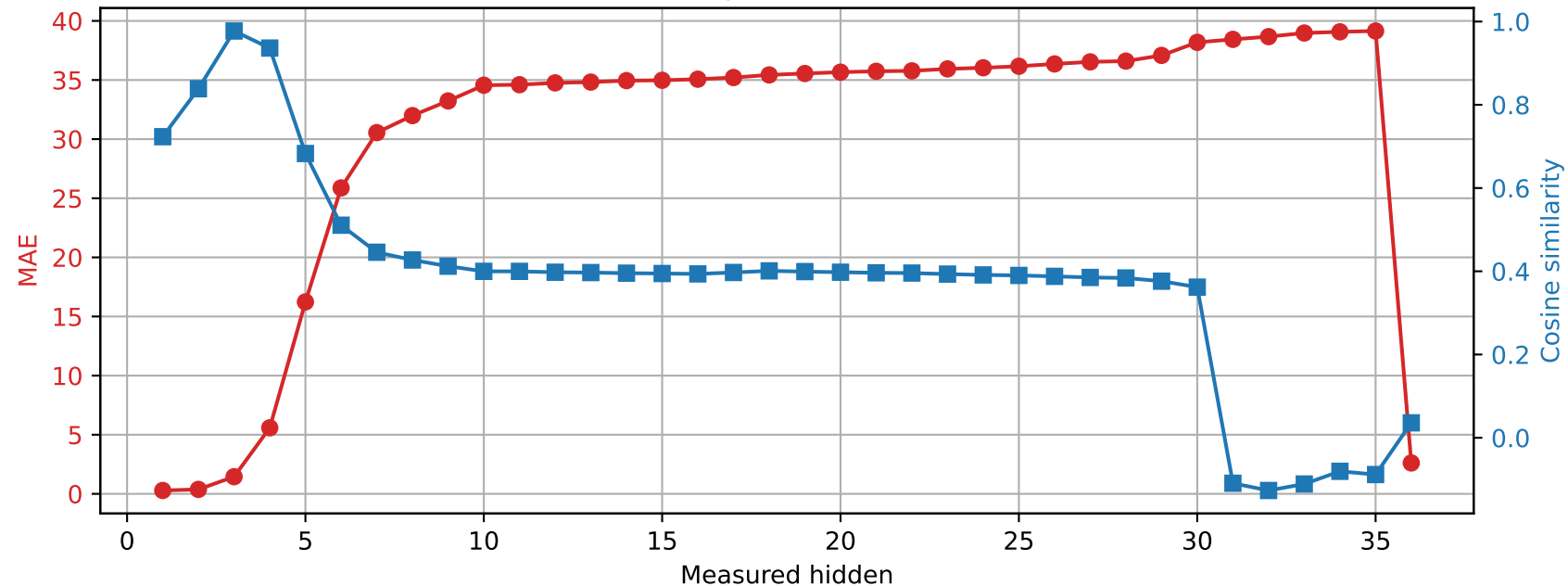
Qwen2.5-3B | Prompt 4 Spared layer 1 | Unquantized vs hybrid
