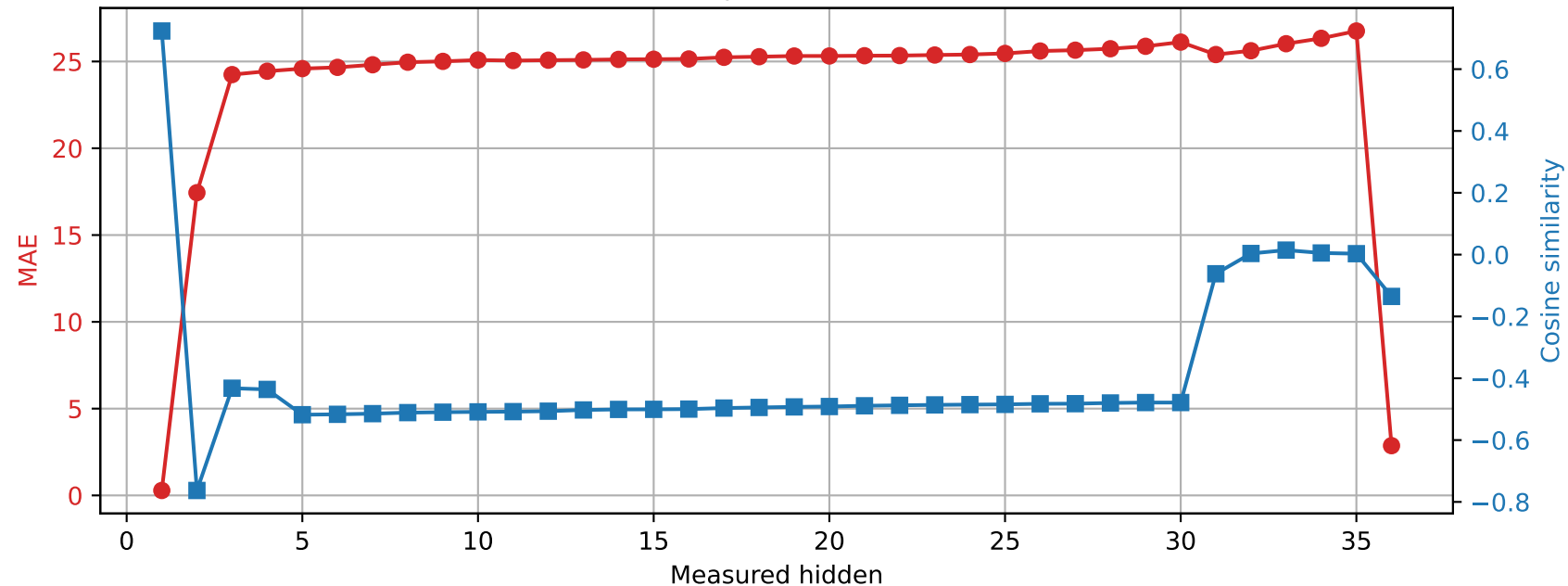
Qwen2.5-3B | Prompt 4 Spared layer 10 | Unquantized vs hybrid
