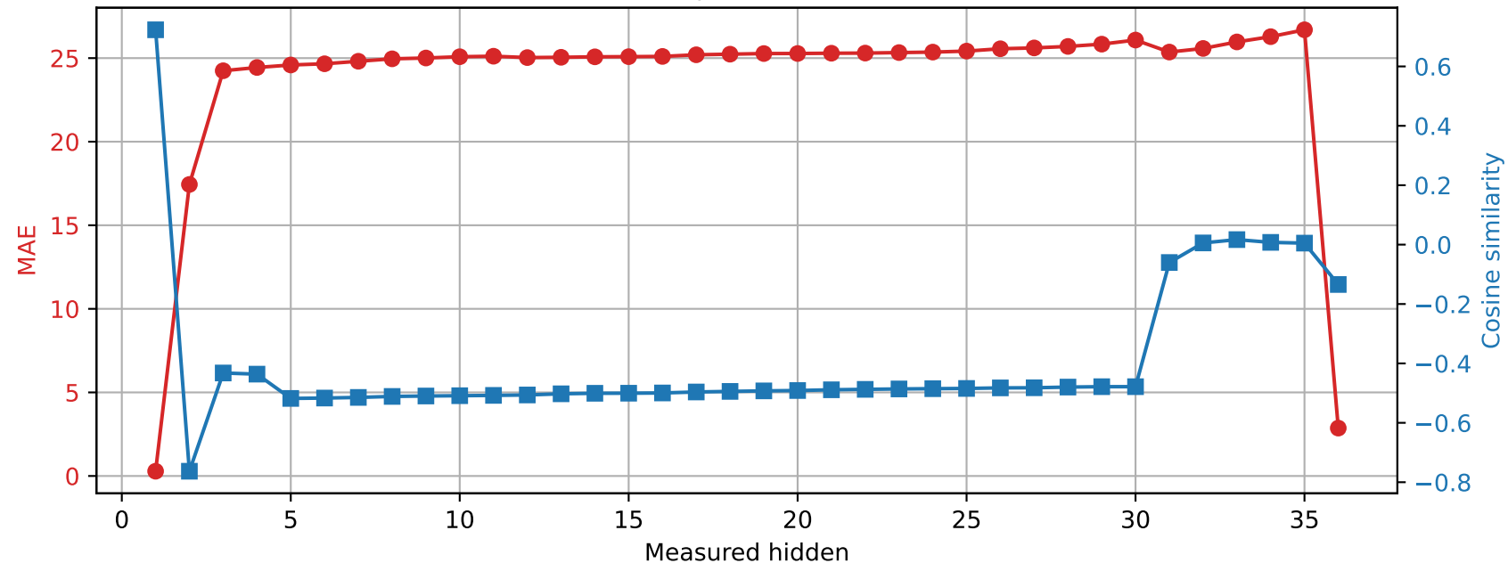
Qwen2.5-3B | Prompt 4 Spared layer 11 | Unquantized vs hybrid
