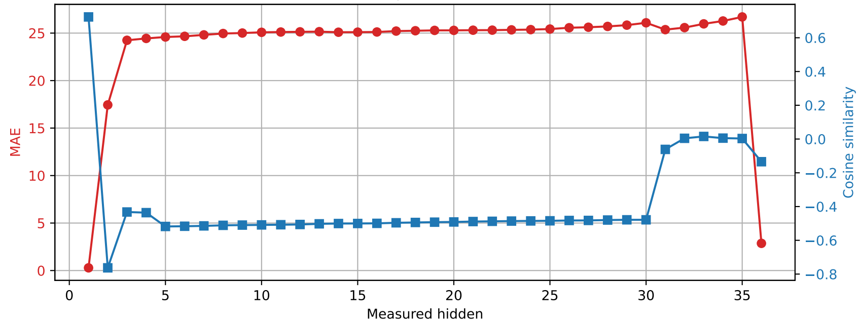
Qwen2.5-3B | Prompt 4 Spared layer 13 | Unquantized vs hybrid
