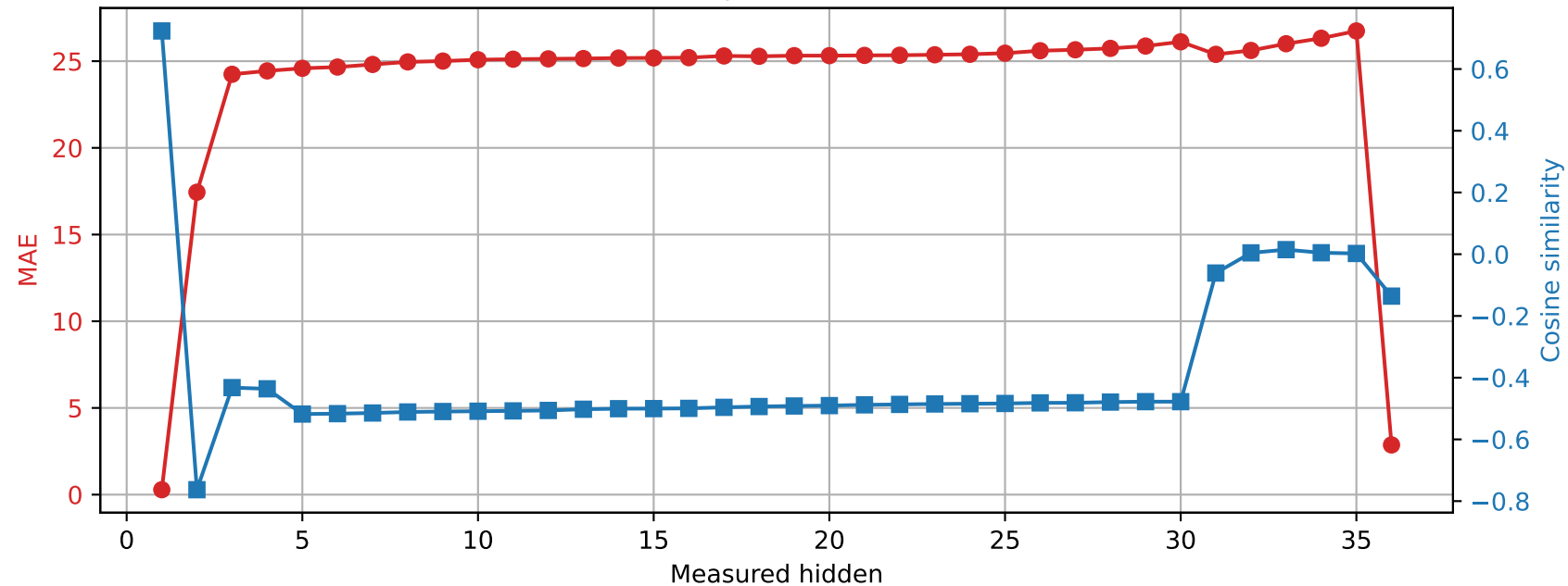
Qwen2.5-3B | Prompt 4 Spared layer 17 | Unquantized vs hybrid
