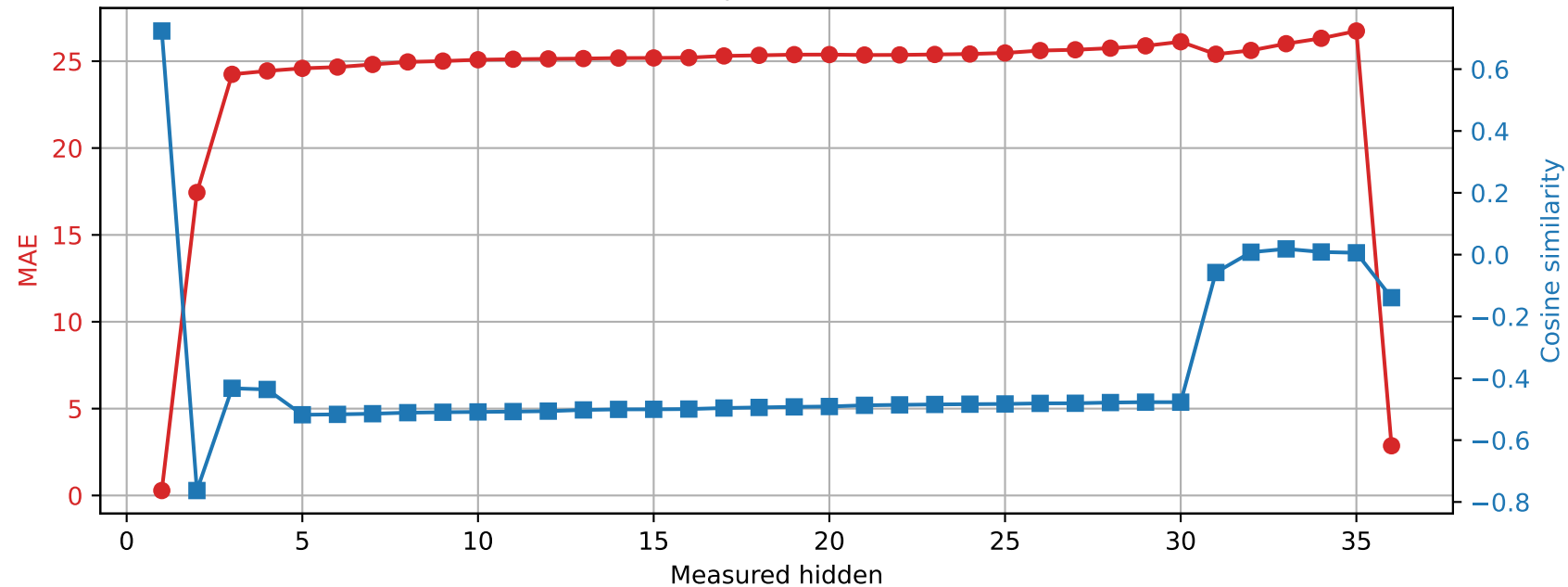
Qwen2.5-3B | Prompt 4 Spared layer 20 | Unquantized vs hybrid
