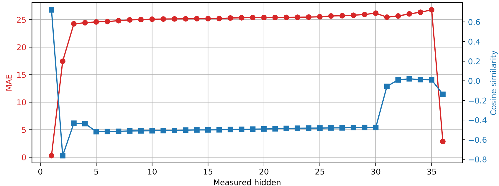
Qwen2.5-3B | Prompt 4 Spared layer 21 | Unquantized vs hybrid
