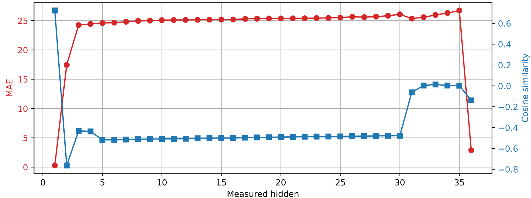
Qwen2.5-3B | Prompt 4 Spared layer 26 | Unquantized vs hybrid
