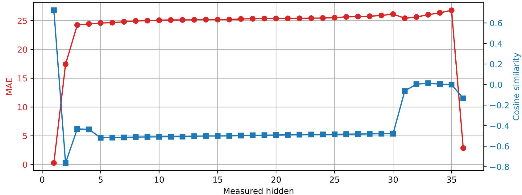
Qwen2.5-3B | Prompt 4 Spared layer 27 | Unquantized vs hybrid
